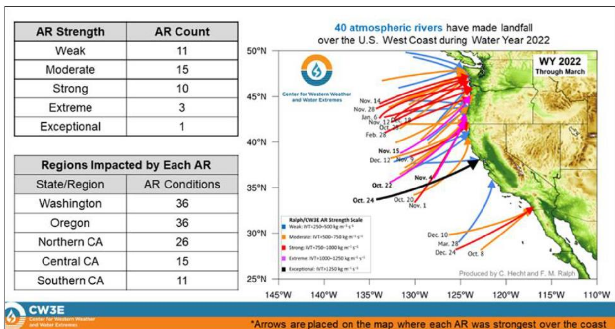
Figure 4-43 2022 Atmospheric Rivers by Strength and Count
