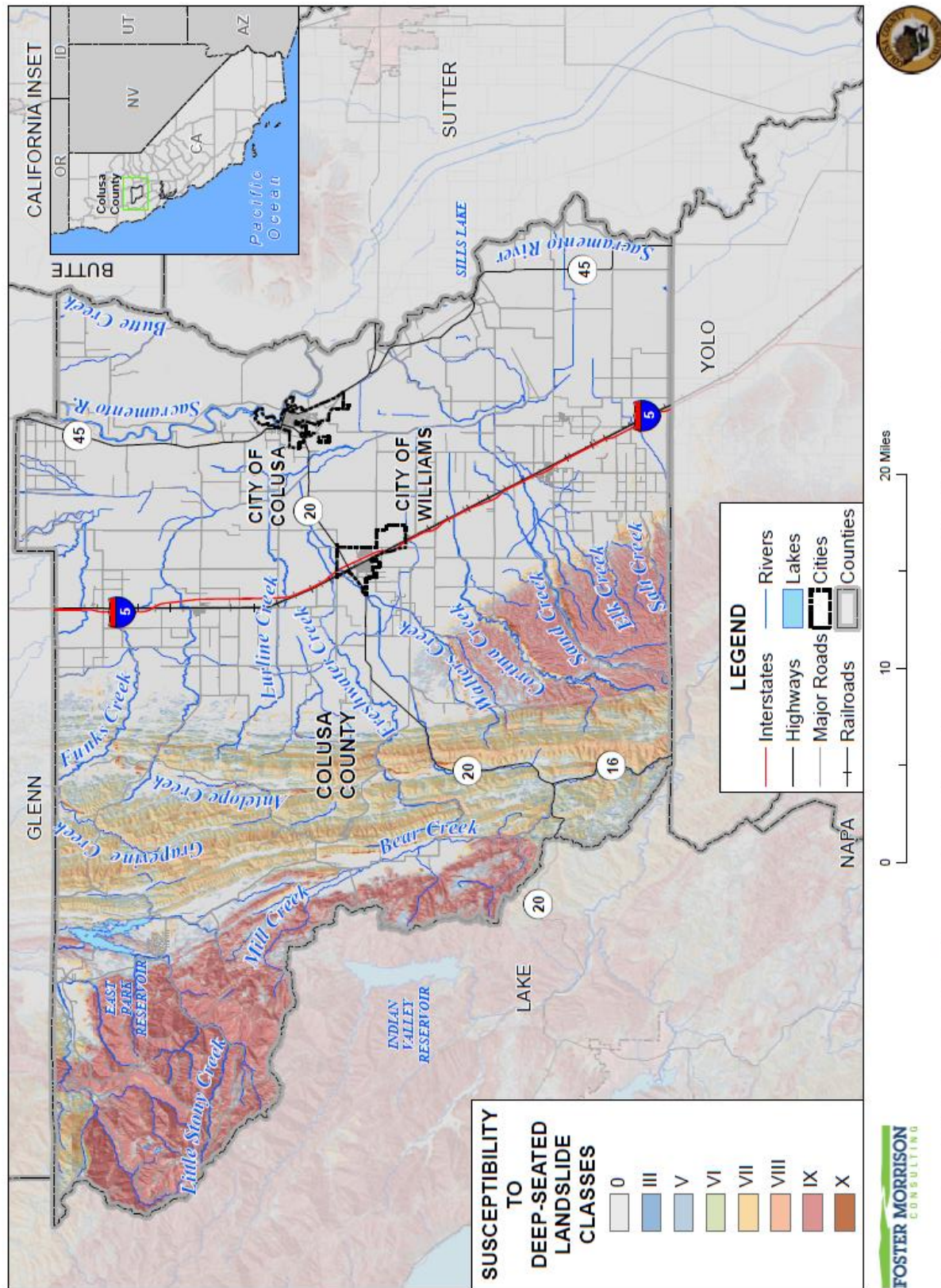
Figure 4-85 Colusa County Planning Area – Susceptibility to Deep Seated Landslides
