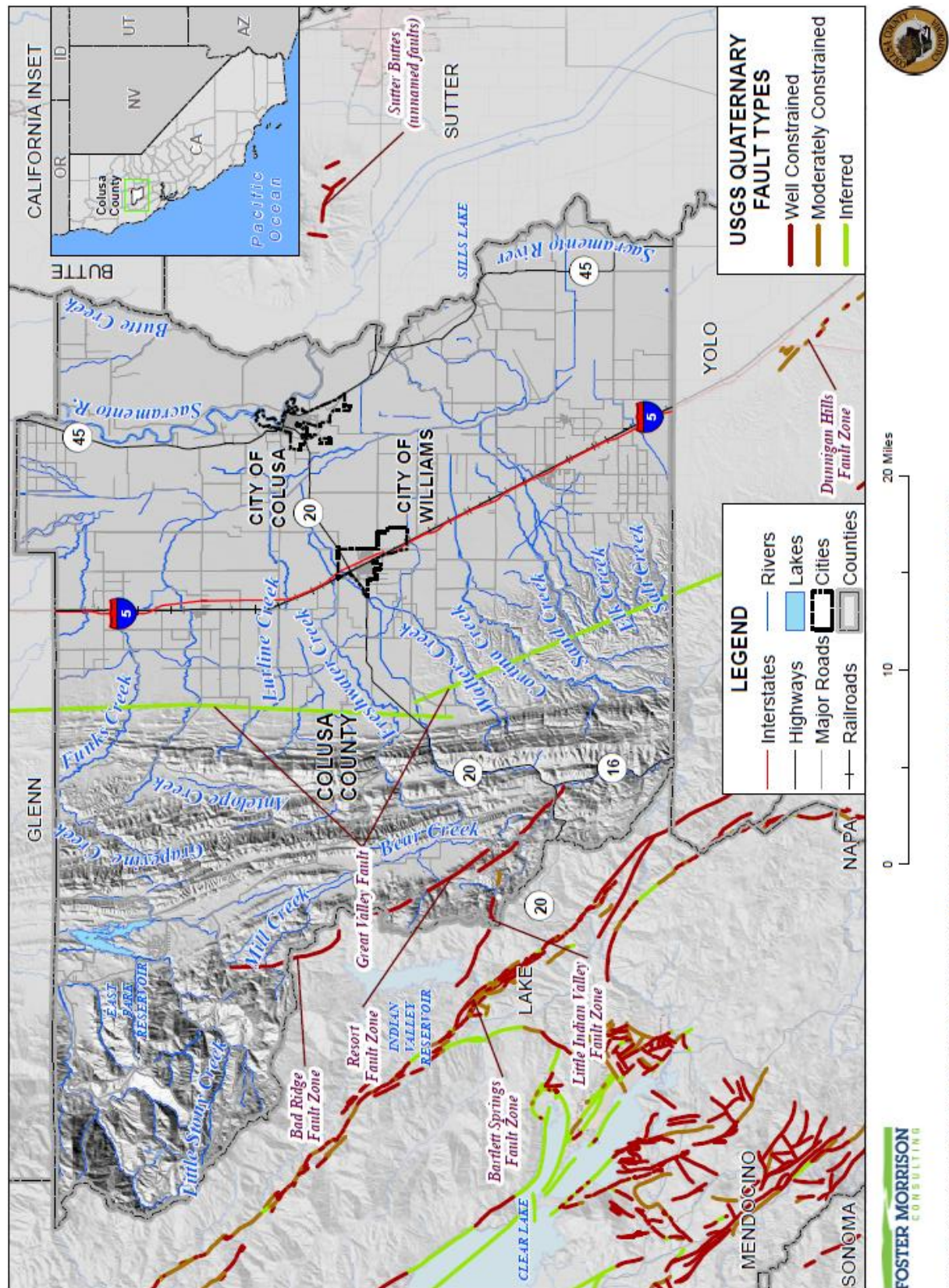
Figure 4-66 Faults in and near Colusa County
