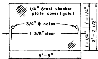
COVER PLAN (WT. 74 lbs)
