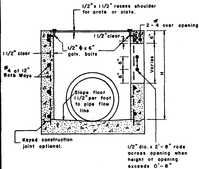
SECTION E-E
