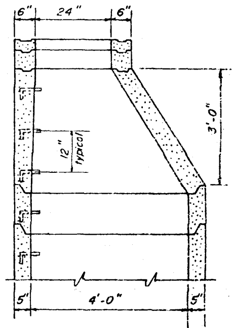
SECTION THROUGH ECCENTRIC TAPER
