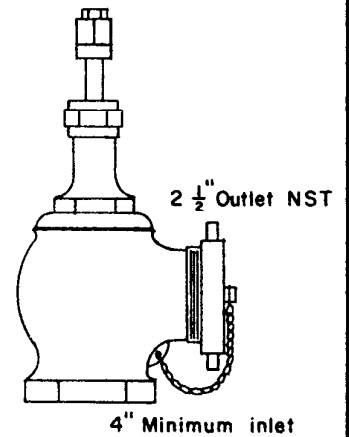
WHARF HYDRANT
