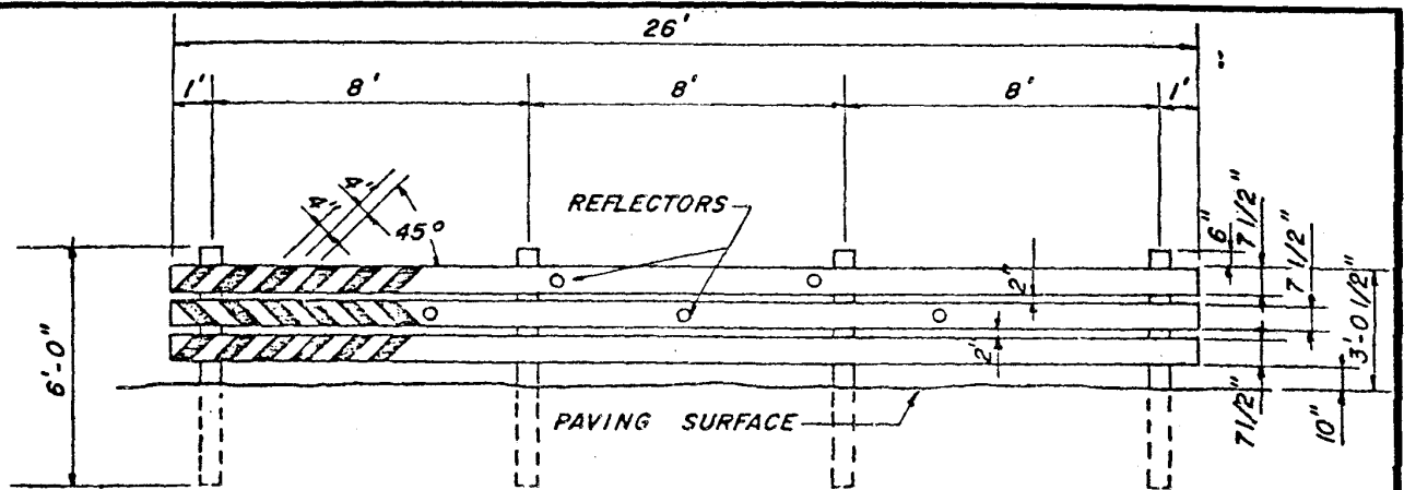
FRONT VIEW
